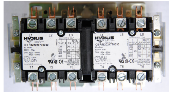
Forward Reverse Contactor Part # 2024778030
