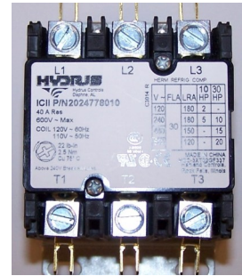
3-Pole Contactor Part # 2024778010
